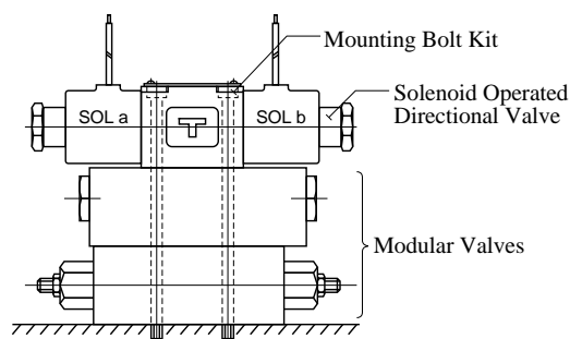
005 Series Modular Valves
